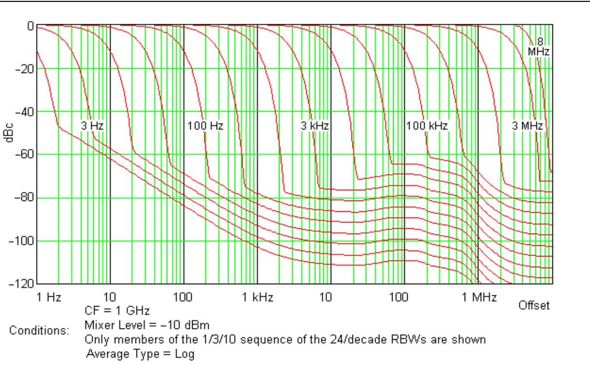
Nominal Dynamic Range vs. Offset Frequency vs. RBW [Plot] (Option 503/507)
